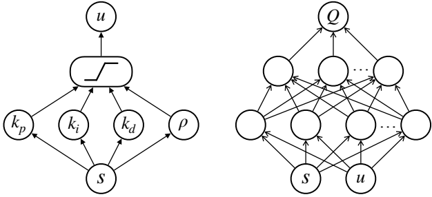
Fig. 1. The actor (PID controller) on the left is simply linear combination of the state and the PID & anti-windup parameters followed by a nonlinear saturation function. The critic on the right is a deep neural network approximation of the Q -function whose inputs are the state-action pair generated by the actor.
